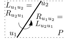
Figure 4. As the A-balanced split rotates, the sectors swap places
