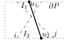
Figure 6. Two canonical chords (dashed) and points u_1, u_2 in the intervals I_1 and I_2 = (i, j) on \partial P . If AL(u_1 u_2) > AR(u_1 u_2) , the next candidate location for u_2 = v(u_1) is tried clockwise of the current u_2 ; otherwise, the search for u_2 , delivering A(u_1 u_2) = 0 , continues counterclockwise
