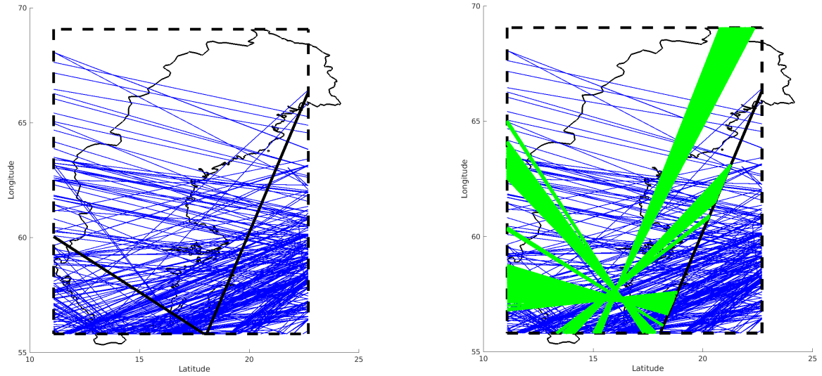
Figure 8. Left: The two cuts meet in a high-degree vertex. Right: Any cut within a green area is doubly-balanced
