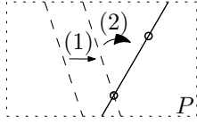
Figure 3. C (dashed) is moved (1) and rotated (2) until becoming canonical (bold). Circles are critical points
