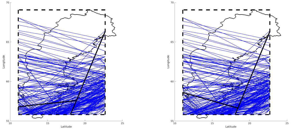
Figure 9. Possible splits
